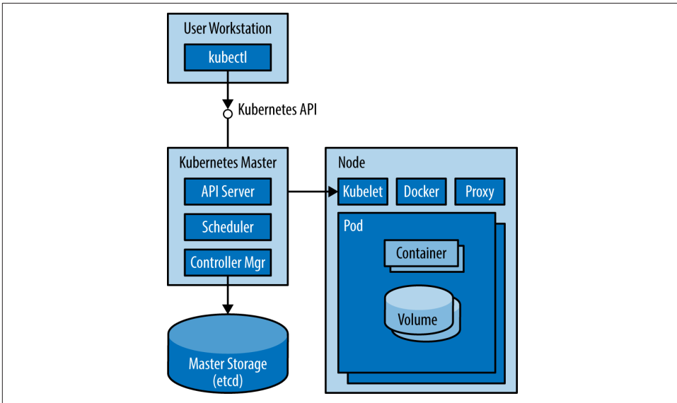
Figure 5-1. Kubernetes architecture
